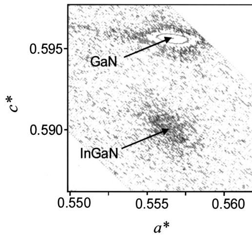
FIG. 1. Reciprocal-space map of x-ray diffraction intensity, in the vicinity of the (204) reflection, for the \text{In}_x\text{Ga}_{1-x}\text{N}/\text{GaN} sample.
