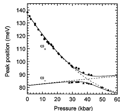
FIG. 6. Comparison of the energies predicted by the two-level anticrossing model discussed in the text with observed data. The dashed curves are the unperturbed energies of the 1s to 2p_{\pm} electronic transition and a two-phonon mode. The solid curves are the perturbed energies calculated from Eq. (5). The circles and triangles are the experimentally measured frequencies of the relevant absorption lines.
