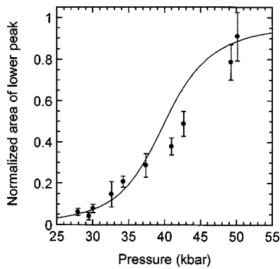
FIG. 7. Pressure dependence of the area of peak III. The circles are the measured peak areas normalized to the area of the 1s to 2p_0 electronic transition peak. The curve is calculated from Eq. (7), assuming that the oscillator strengths of both electronic transitions are equal to each other at all pressures.
