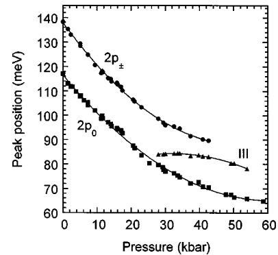
FIG. 4. Pressure dependence of the electronic transition peaks in AISb:Se. A third peak (indicated by the triangles and labeled III) begins to appear at about 30 kbar. The lines are included as guides to the eye.
