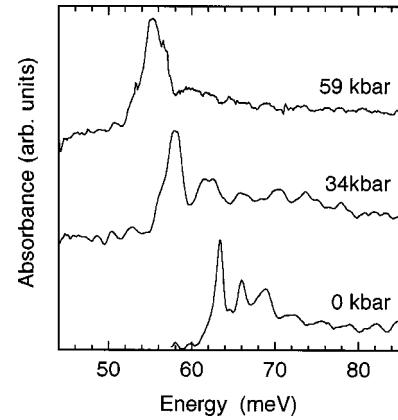
FIG. 1. Absorption spectra of AlSb:Te at three different hydrostatic pressures. The largest single peak is assigned to the 1s to 2p_{\pm} electronic transition.
