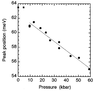
FIG. 2. Energy of the 1s to 2p_{\pm} transition line in AlSb:Te as a function of pressure. Pressures for the two square points were measured in situ at low temperature while pressures for the points indicated by circles were measured at room temperature. The line is a linear fit to the high-pressure points.
