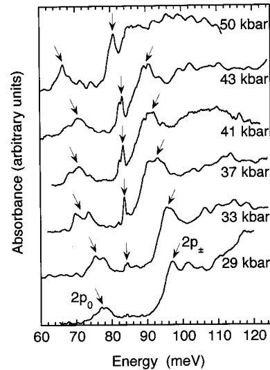
FIG. 5. Spectra of AlSb:Se showing the emergence and growth of the third peak as the pressure is increased. The slanted arrows indicate the 1s to 2p_0 and 1s to 2p_{\pm} electronic transitions, and the vertical arrows point to the emerging third peak. At 50 kbar, the emerging peak resembles the original 1s to 2p_{\pm} electronic transition peak (compare with the spectra in Fig. 3).
