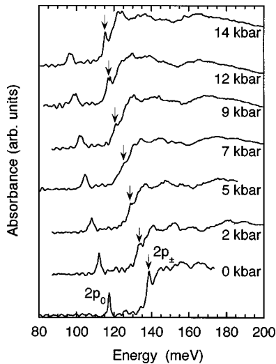
FIG. 3. AISb:Se donor spectra at low pressures showing the disappearance and reemergence of the 1s to 2p_{\pm} electronic transition peak. The higher-energy peak nearly disappears into the continuum around 7 kbar, then reappears as the pressure is increased further. The vertical arrow tracks the 1s to 2p_{\pm} electronic transition.
